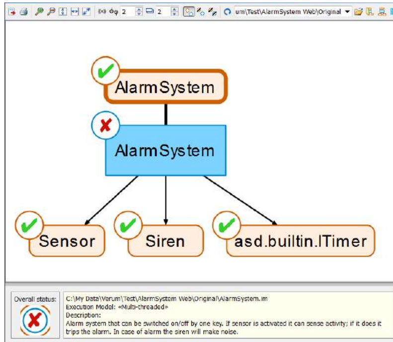
Model Navigator
